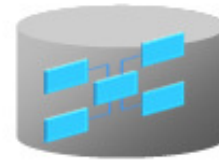
Data Warehouse
